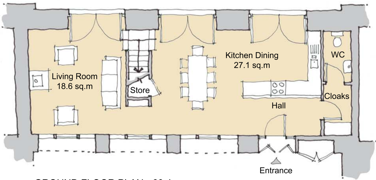
GROUND FLOOR PLAN - 60.4 sq.m
