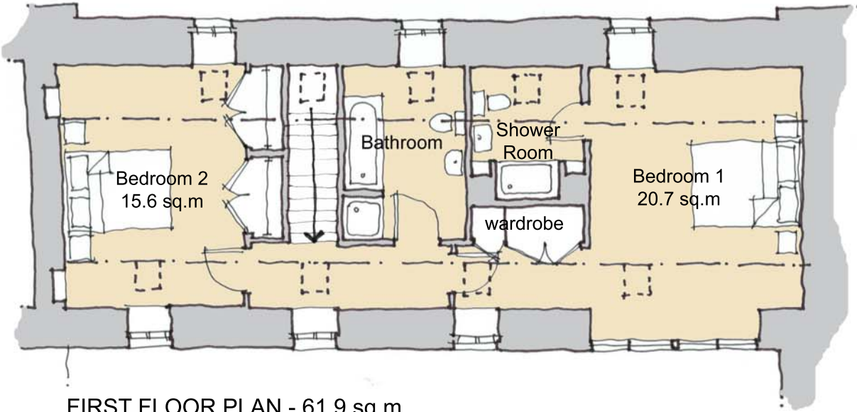
FIRST FLOOR PLAN - 61.9 sq.m
